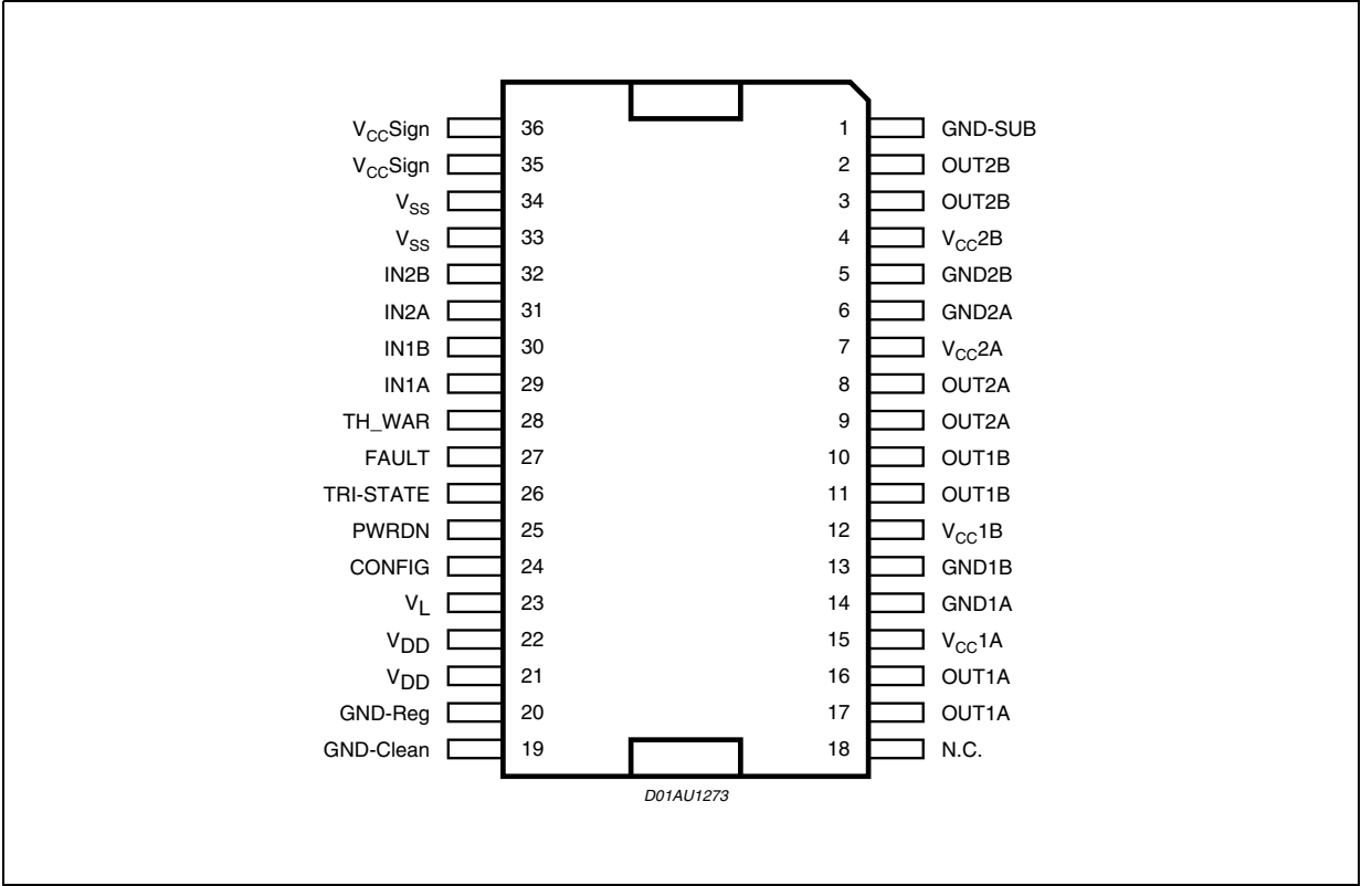
Figure 3. PIN CONNECTION
